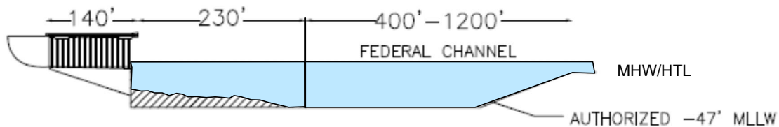
2-2 TYPICAL SECTION AT BERTH #2
