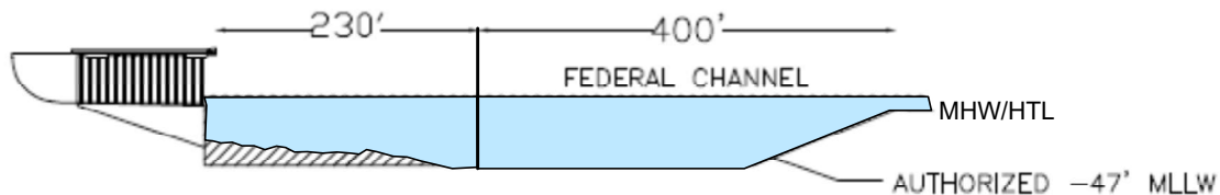
2-1 TYPICAL SECTION AT BERTH #1
