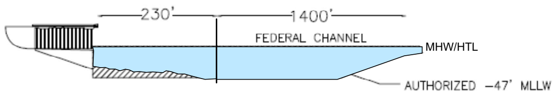
2-3 TYPICAL SECTION AT BERTH #3
